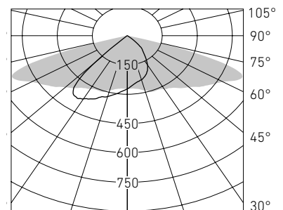
FREGAT LED 110 5000K
